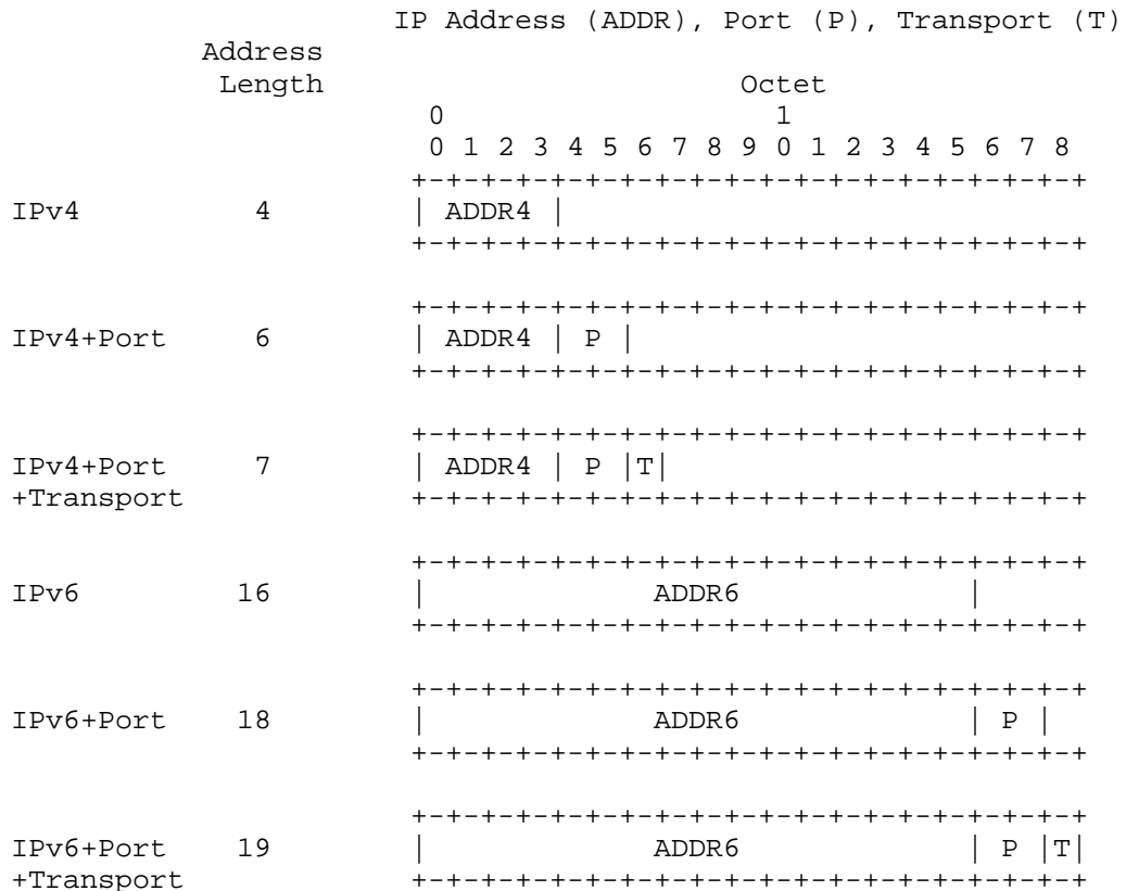
Figure 1: Encoding of the Native IP Addresses for ANSI C12.22
